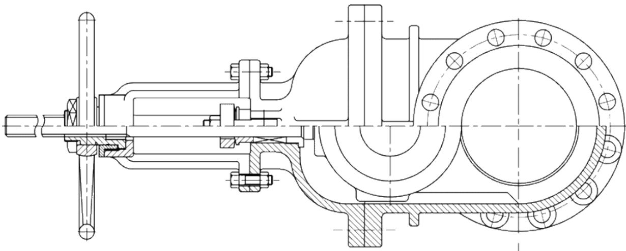
Rising Stem Gate valve
